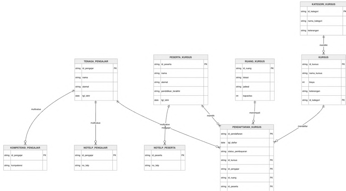
Gambar 2 Gambar Model Relasional
